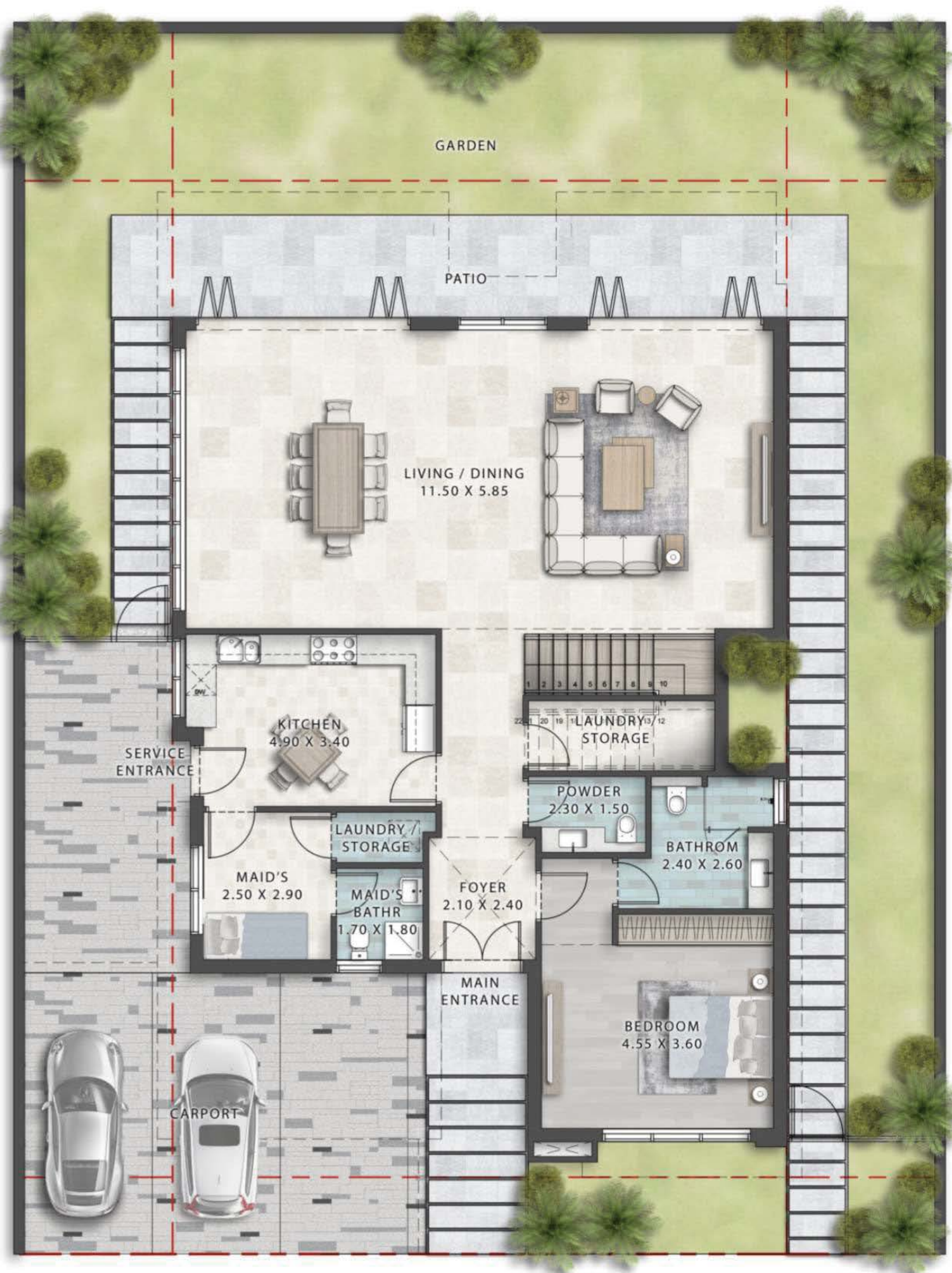
GROUND FLOOR
