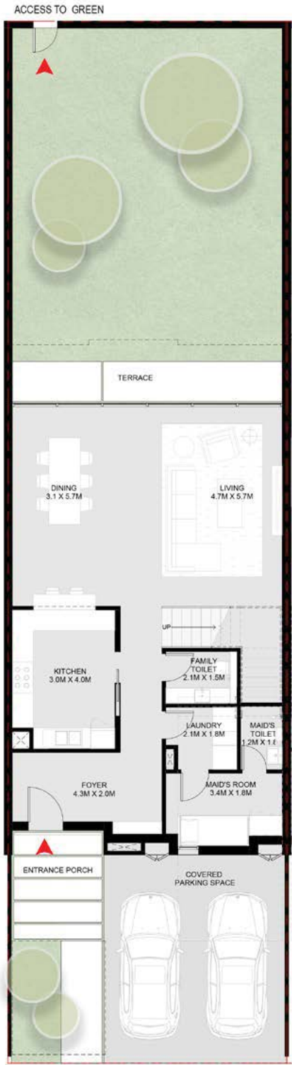
Ground floor
