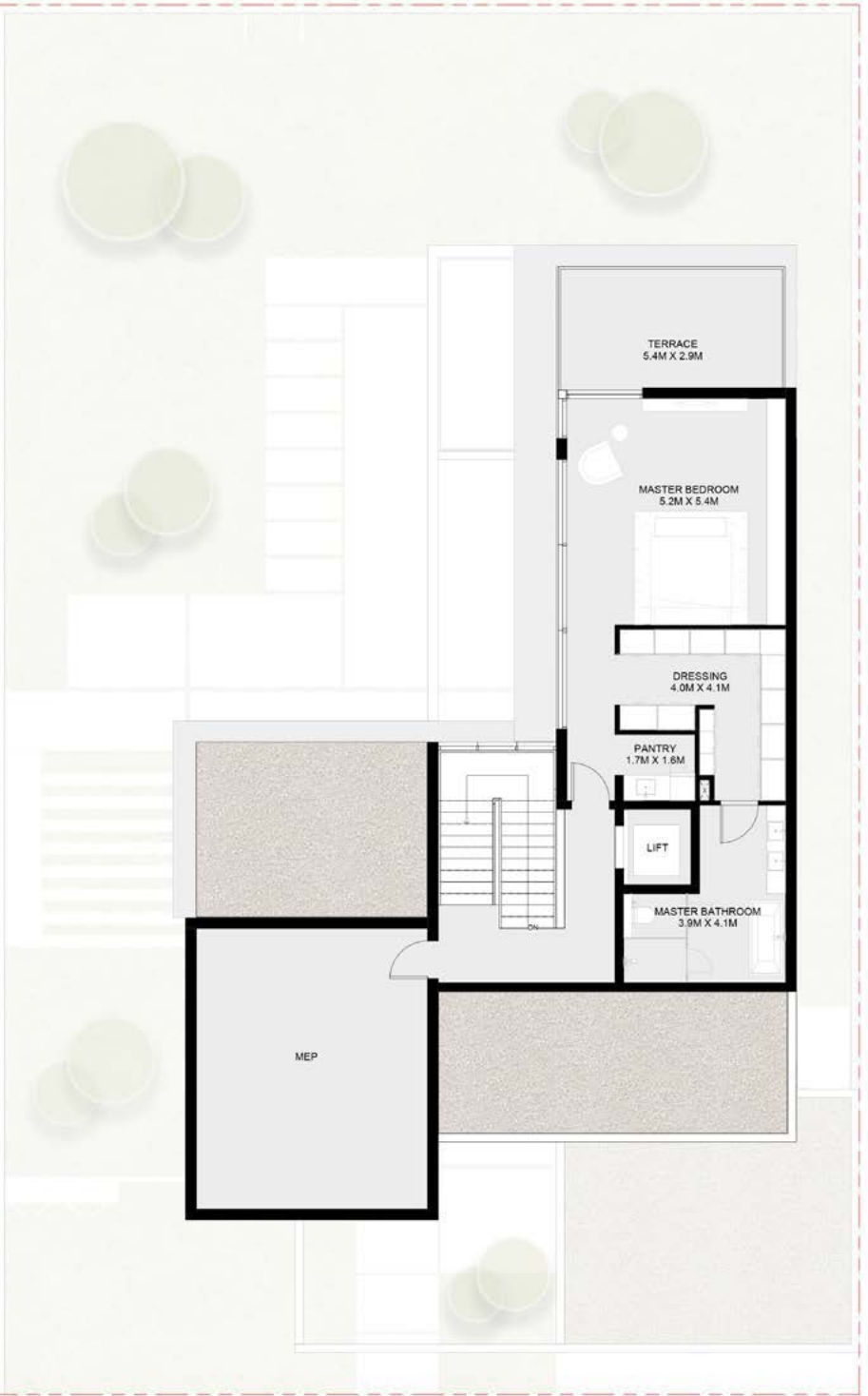
Second floor
