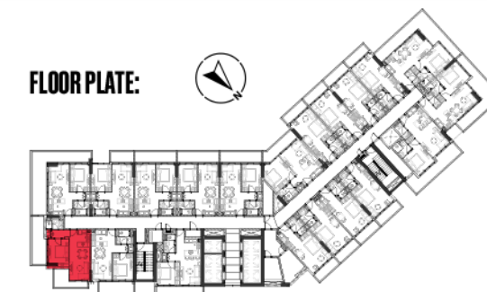
Floors 03 - 09
