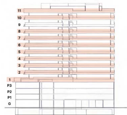
KEY SECTION
