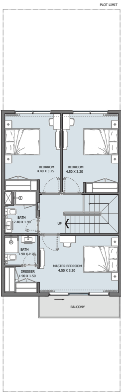
1ST FLOOR
